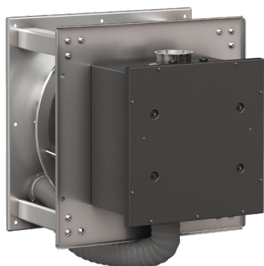
EC centrifugal fans – RadiPac with motor enclosure and hose for food service sector Fan sizes 400, 450, and 500
